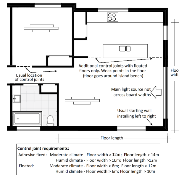
Figure 2 – Installation
