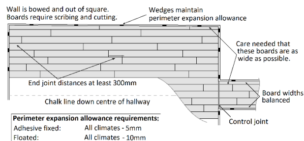
Figure 3 – Scribing
